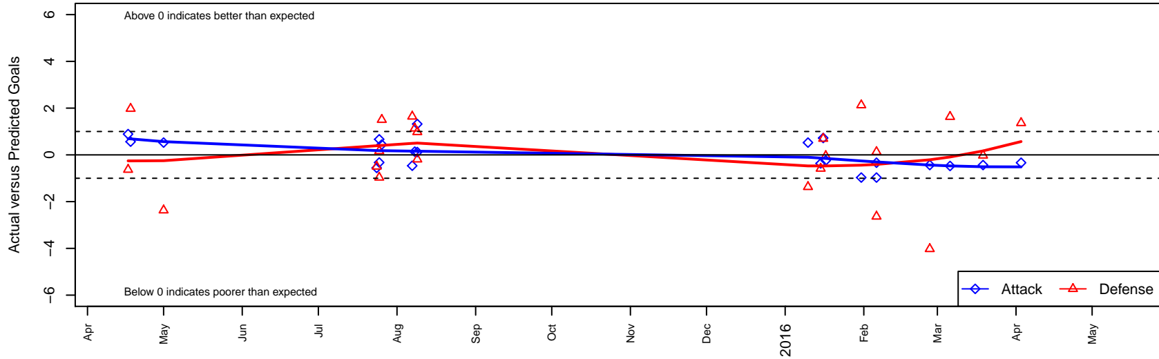
PS Slammers Black G98 Dots are actual minus expected GF (blue circles) and GA (red triangles). Blue line is smoothed change in attack strength. Red is smoothed change in defense strength.
